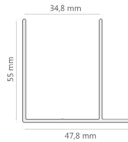
Expansor D-2055
