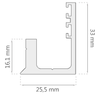
U P-5105/8
