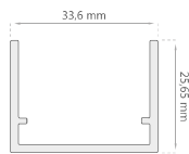
Expansor D-2098
