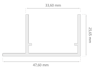
Bisagra Pivoteante
