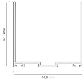
Expansor D-2012
