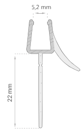
C-1203/6
